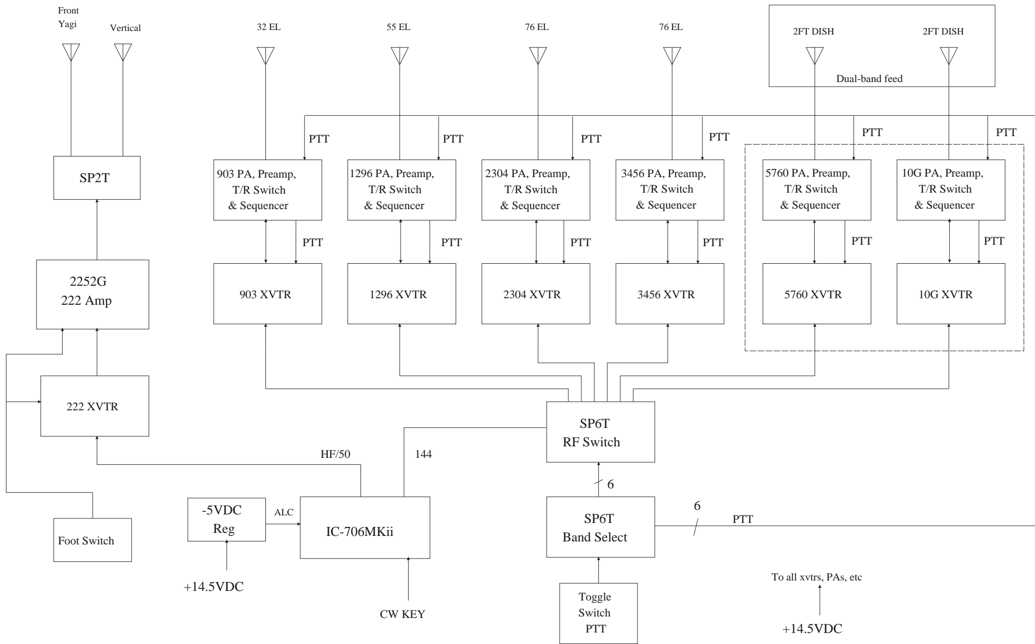
W3IY/R Microwave System Block Diagram
